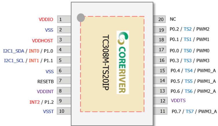
TC308M-TS20IP Package Diagram
